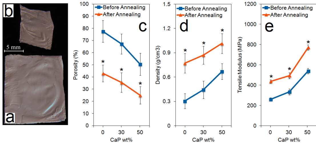
Figure 4.2 Effect of heat treatment on the aligned nanofiber microsheets shrinkage before heating (a) and after heating (b). The effect of heat shrinking on porosity(c), density(d) and tensile modulus(e). Experimental groups include GLU-NF, GLU-NF/CaP30, GLU-NF/CaP50, and GLU-NF/LBL200. One star indicates statistically significant difference (s.d.; p < 0.05 ) between before annealing and after annealing for the same experimental group. Error bars correspond to means \pm 1 SD for n = 3 .
